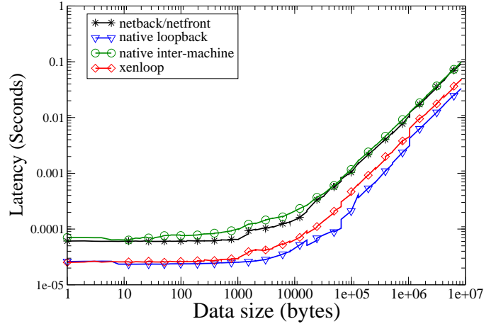
Figure 7: Latency versus message size for netpipe-mpich benchmark.
