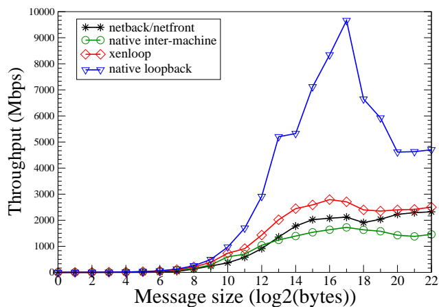
Figure 9: Throughput versus message size for OSU MPI Bi-direction benchmark.
