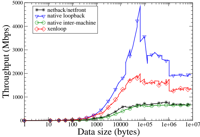
Figure 6: Throughput versus message size for netpipe-mpich benchmark.
