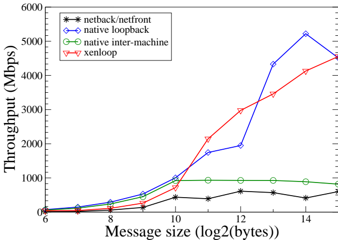
Figure 4: Throughput versus UDP message size using netperf benchmark.
