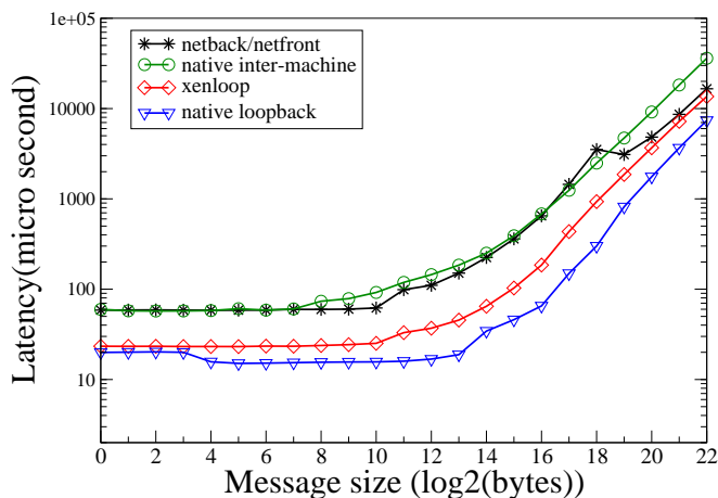
Figure 10: Latency versus message size for OSU MPI Latency benchmark.
