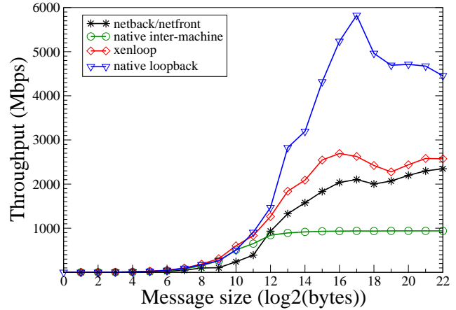
Figure 8: Throughput versus message size for OSU MPI Uni-direction benchmark.
