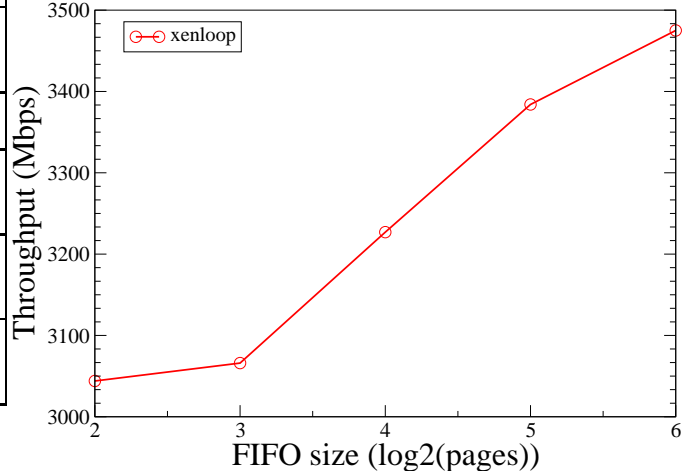
Figure 5: Throughput versus FIFO size using netperf UDP bandwidth test.
